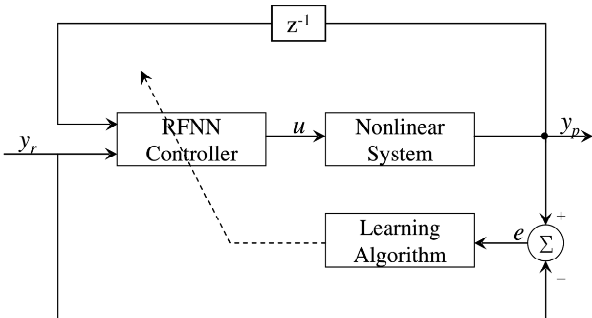
Figure 5: Dynamic System Control Configuration with RFNN Controller
